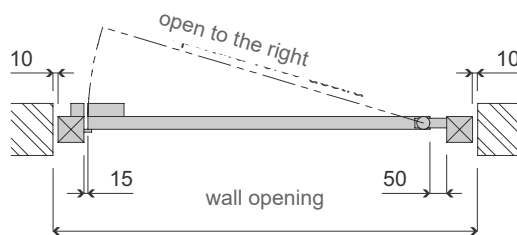
OUTSIDE VIEW
