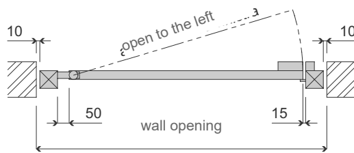
OUTSIDE VIEW
